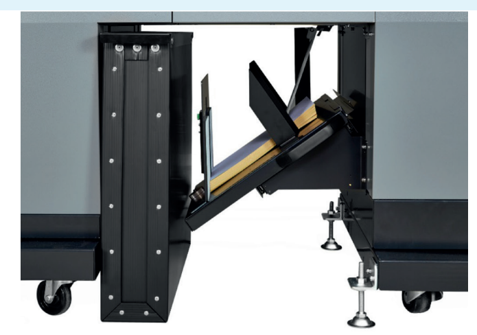
DBM-600: Corner and side stitch tray
